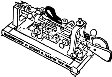
Code-sending bug.
